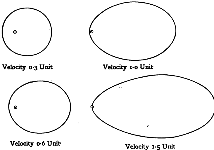
FIG. 5.—Simple Drift Curves.
